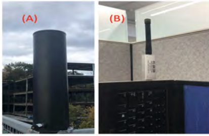
Figure 8: Hardware used in SelfieStick (A) Weather Antenna, (B) RTL SDR with Laird Antenna
