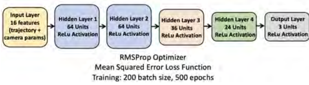
Figure 6: DNN Architecture
